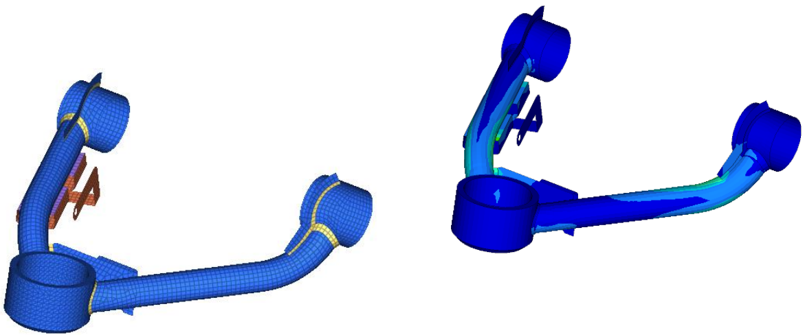
Figure 2: Upper Control Arm Mesh and Stress Contour
