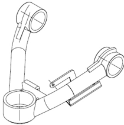
Figure 1: Upper Control Arm Design
